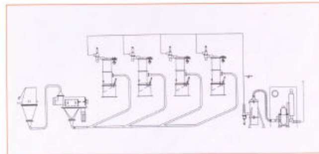
SACK TIPPING, IN-LINE SIEVING AND VACUUM DISTRIBUTION
