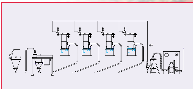
IN-LINE CONE NIBBLER IN VACUUM CONVEYING SYSTEM
